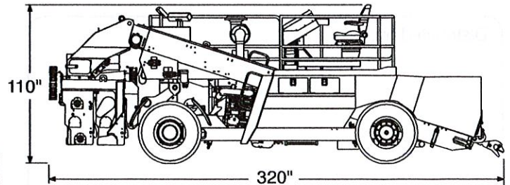
BIG ChipSpreader
